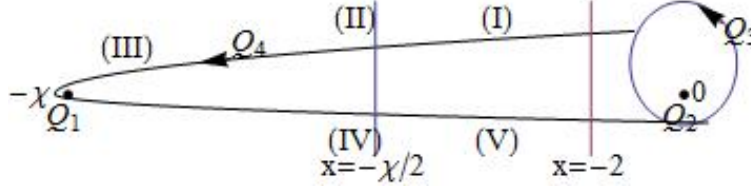
FIGURE 3. Poincaré sections
