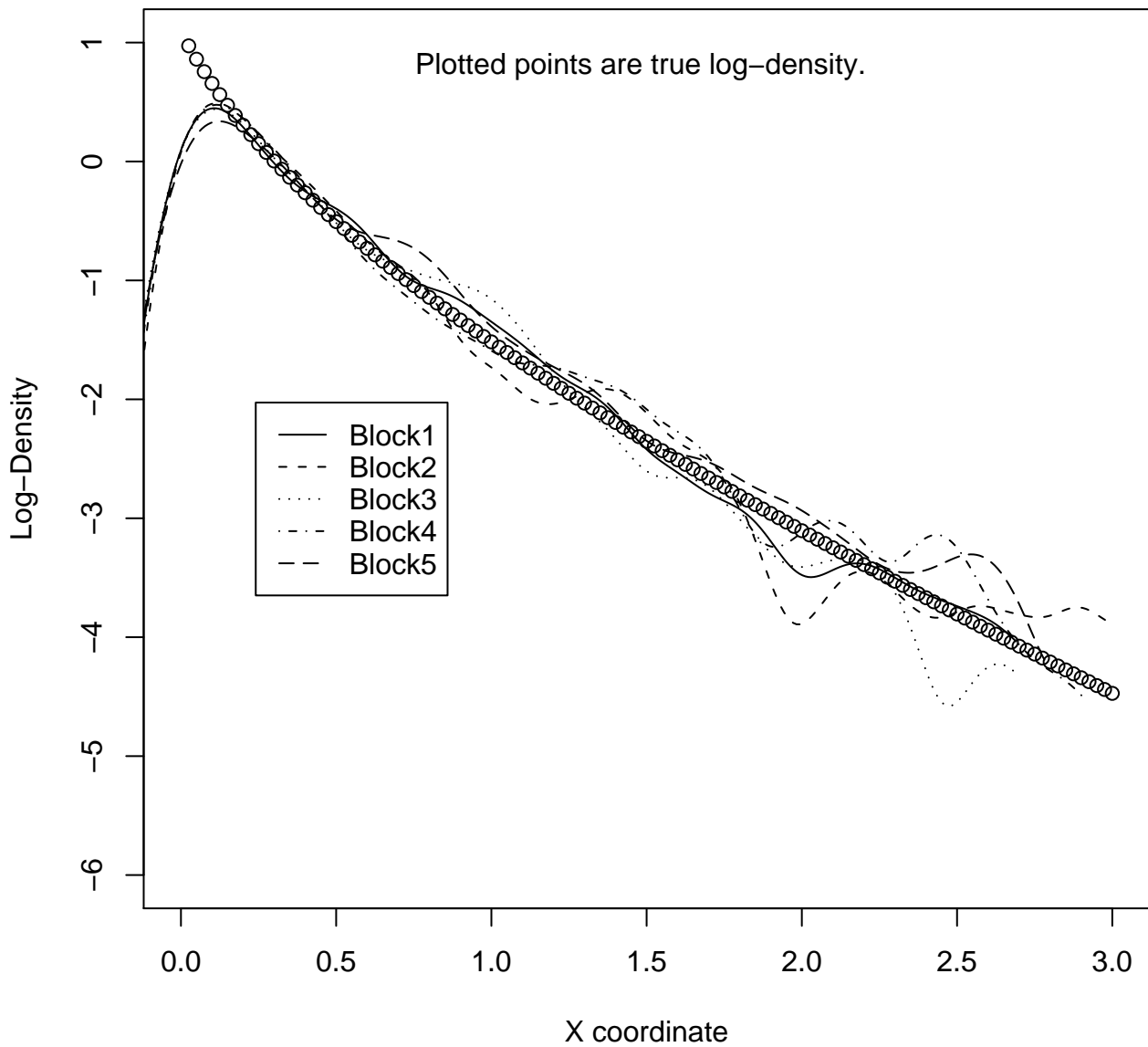
Plot of Log of True Density and Smoothed Hist's for X_t , t=5001,10000 , in blocks of 1000
