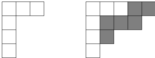
FIGURE 2. A hook and a double hook
