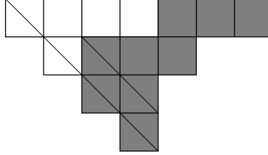
FIGURE 6. The (shifted) double shape (4, 1) \subset (7, 4, 2, 1)
