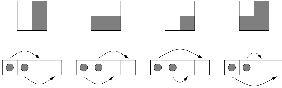
FIGURE 4. Four move pairs with signs +1, +1, -1, -1
