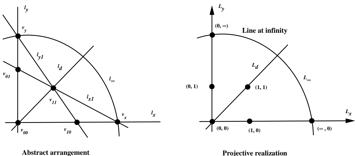
Figure 15: The standard triangle T and its standard realization.
