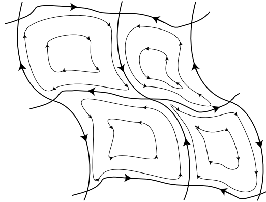
Fig. 1. A period of the cellular flow.
