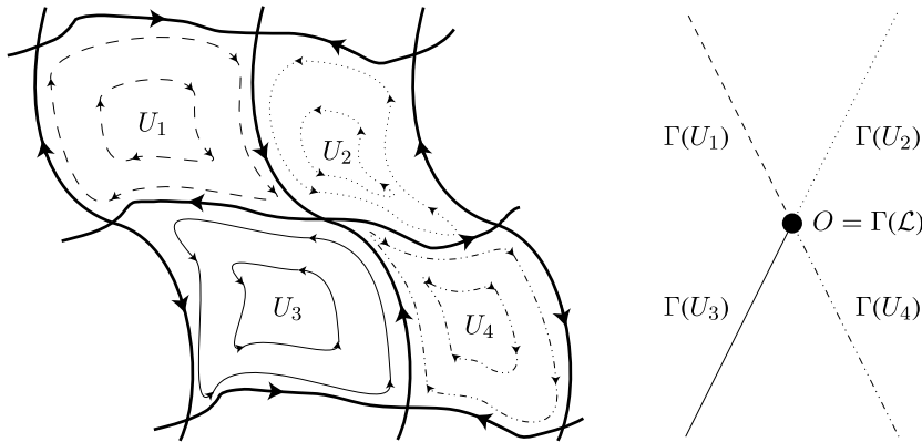
Fig. 2. The graph corresponding to the structure of the level sets of H on \mathcal{T} .
