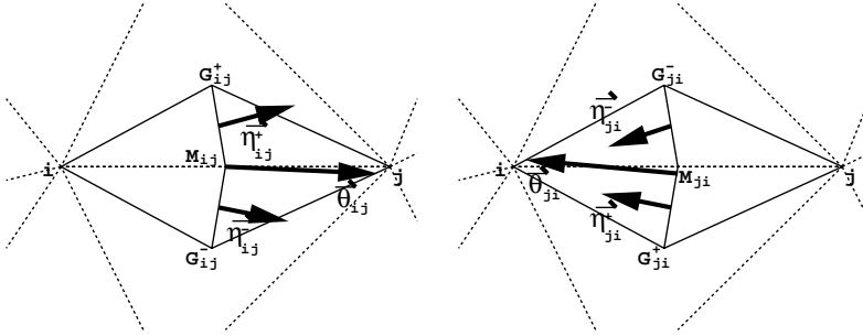
Fig. 2. Normals to C_i and L_{ij}
