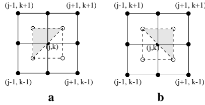
Fig. 3.2a,b. Non-staggered LxF schemes for the H-J equations
