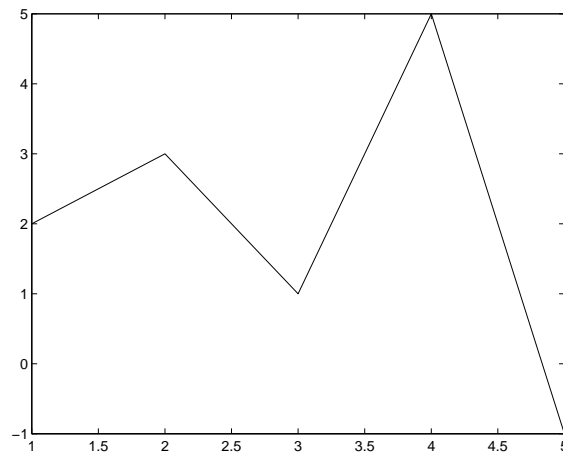
Figure 1.1: Plot \mathbf{x} versus \mathbf{y} for the vectors \mathbf{x} = (1, 2, 3, 4, 5) and \mathbf{y} = (2, 3, 1, 5, -1) .
