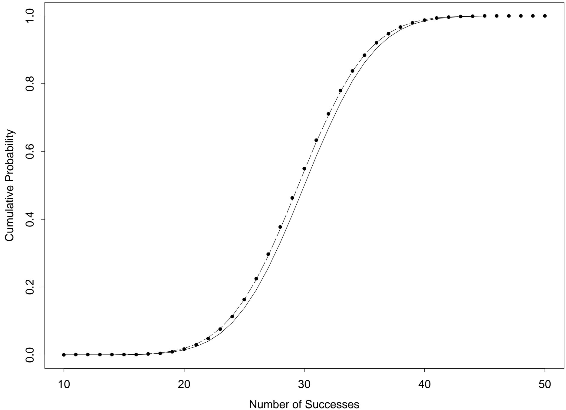
Distribution Functions of Binom(100,.3) (dots) & N(30,21) (line) Dashed line is continuity-corrected curve
