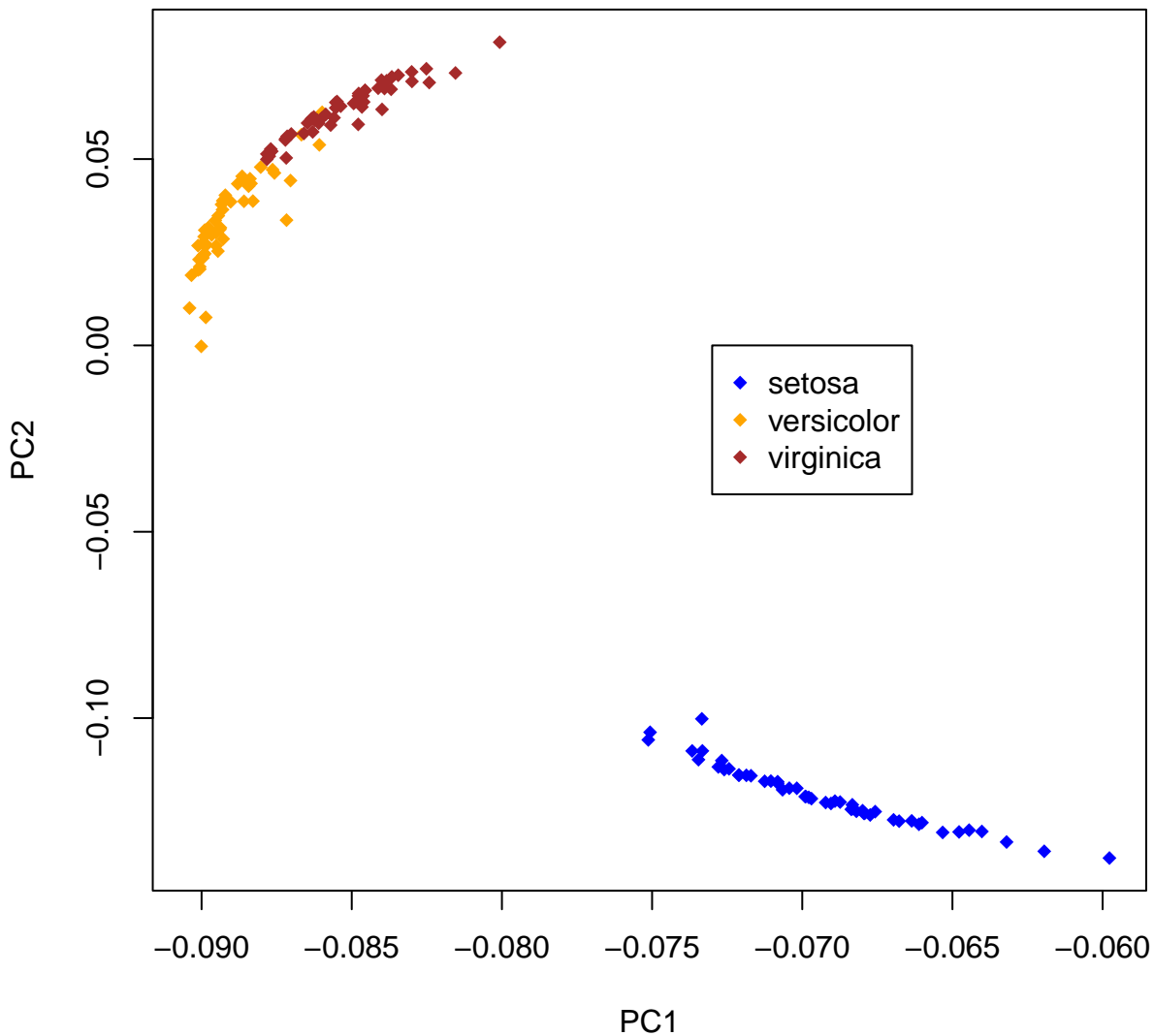
PC plot, Iris Data, Power 6 kernel
