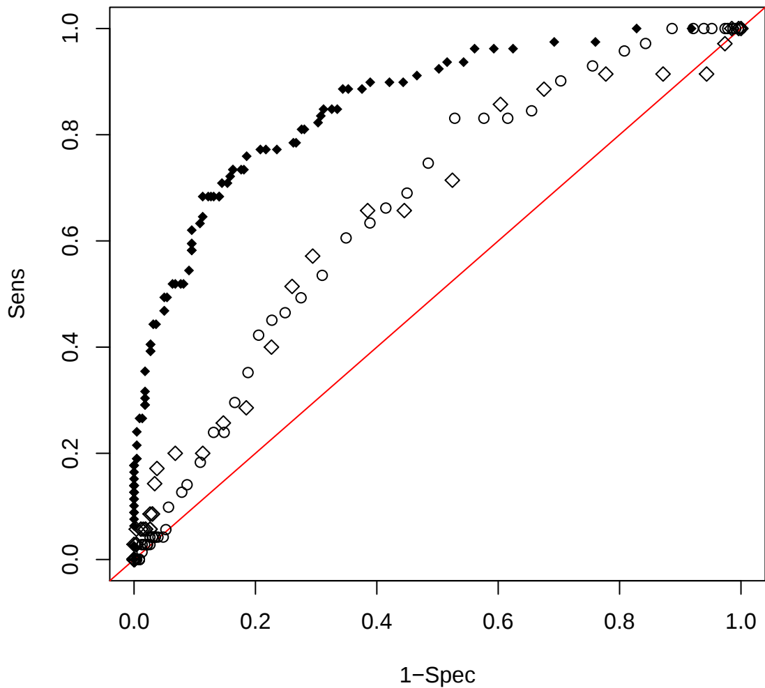
ROC Plot
