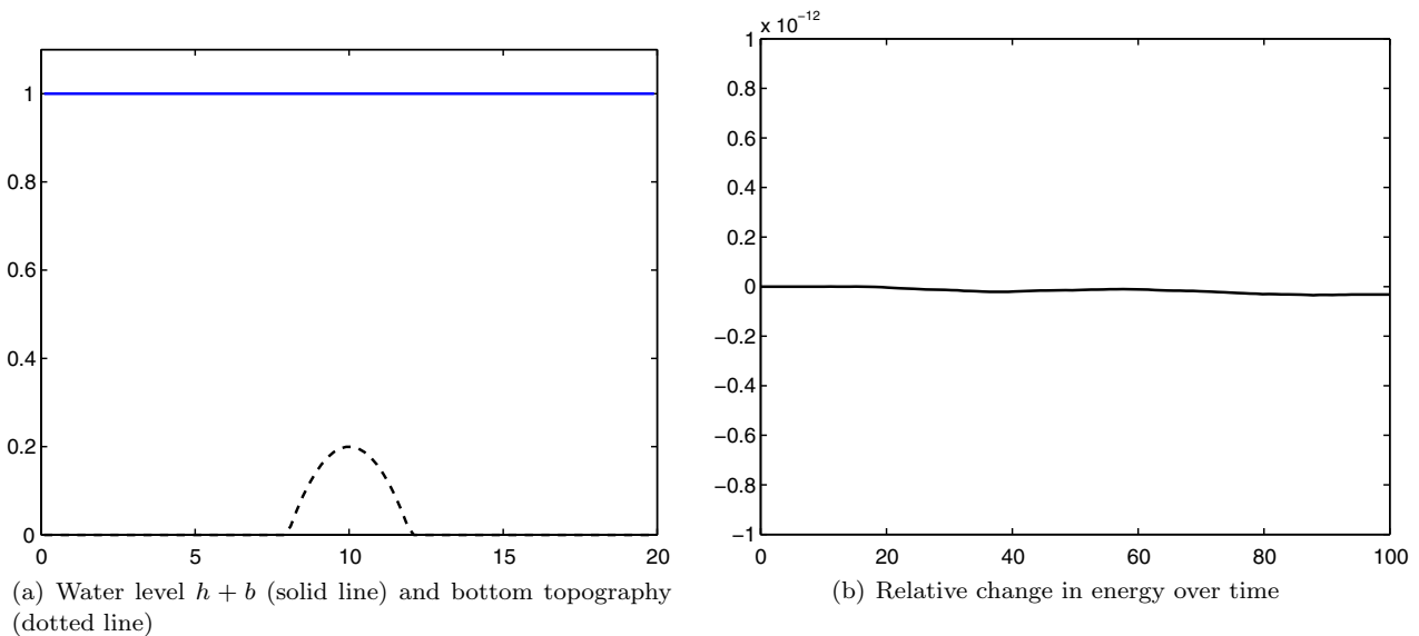
Fig. 2. Lake at rest at t = 100 using 200 mesh points.
