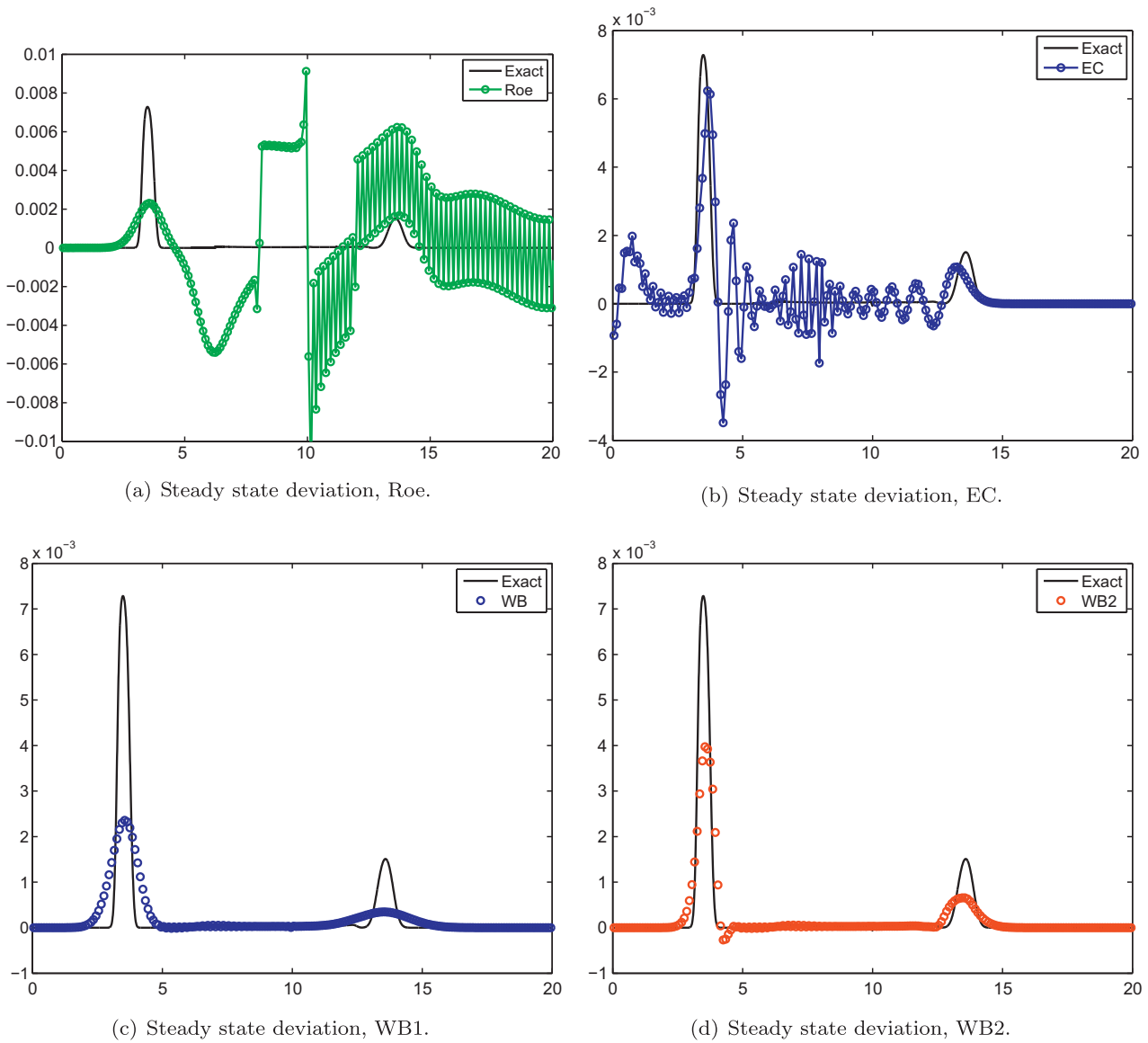
Fig. 10. Perturbed transonic moving steady state at t = 1.5 using 200 mesh points.
