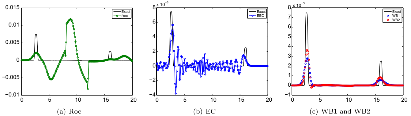
Fig. 8. Perturbed subsonic moving steady state at t = 1.5 .
