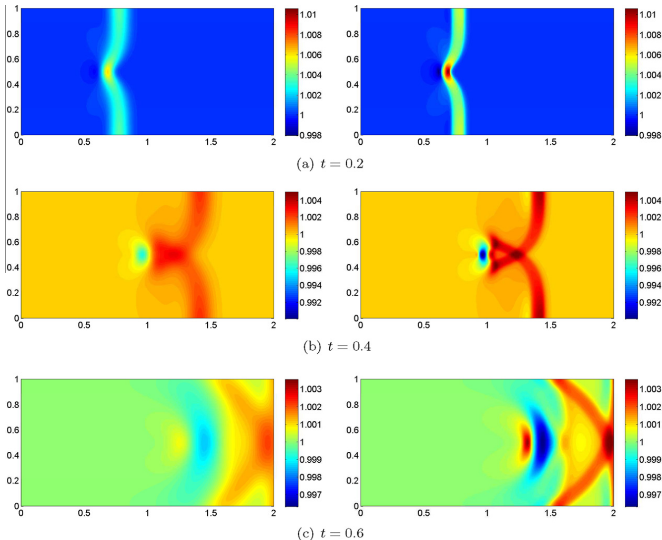
Fig. 12. A simulation of the two-dimensional lake at rest with perturbation using the ES1 and ES2 scheme with 600 \times 300 mesh points. Left column: ES1; right column: ES2.
