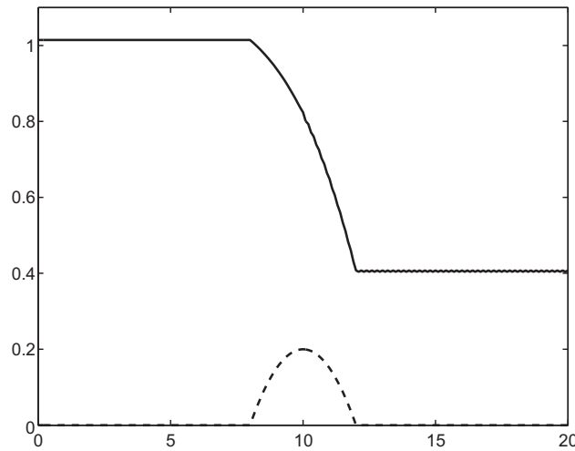
Fig. 9. Initial surface level of the transonic steady state.
