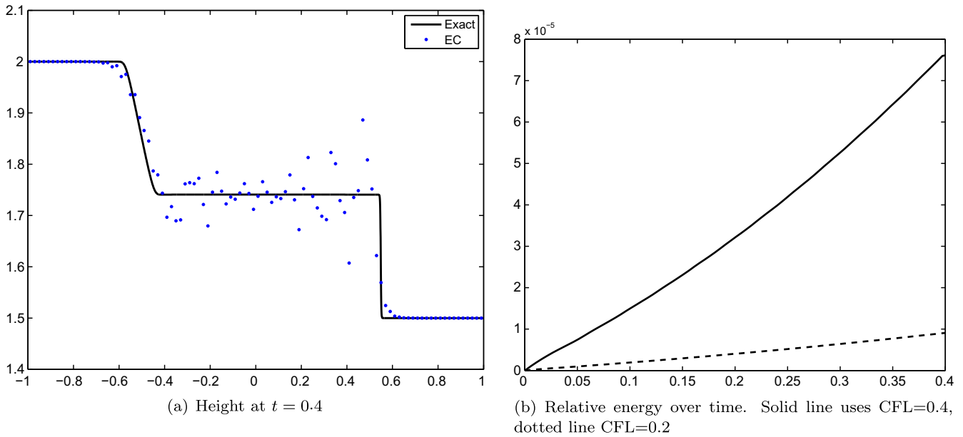
Fig. 1. The EC scheme computes a dambreak problem.
