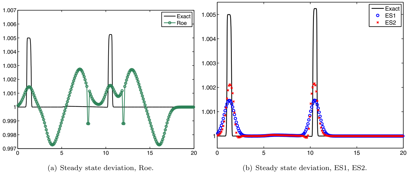
Fig. 5. Lake at rest with perturbation at t = 1.5 on a mesh with 200 mesh points.
