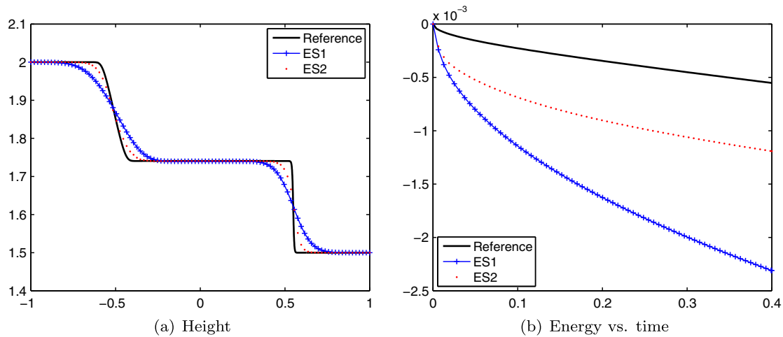
Fig. 4. Solutions computed with the first- and second-order versions of the energy stable scheme, ES1 and ES2 with 100 mesh points.
