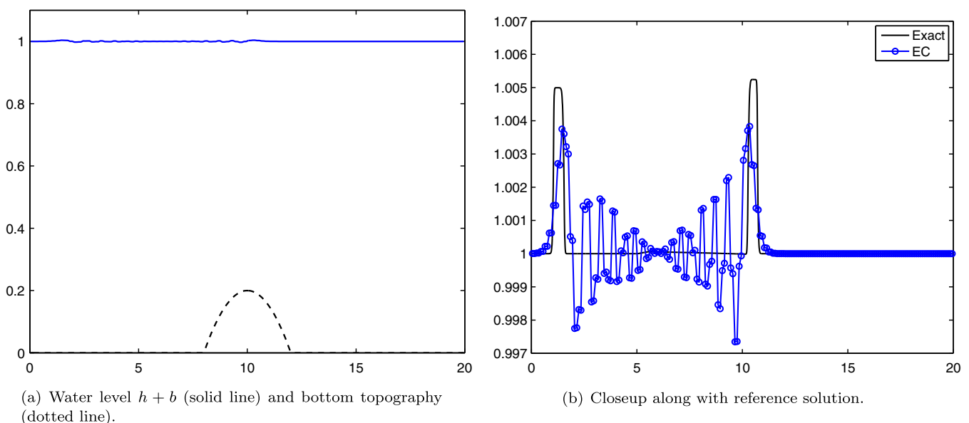
Fig. 3. Lake at rest with perturbation at t = 1.5 .
