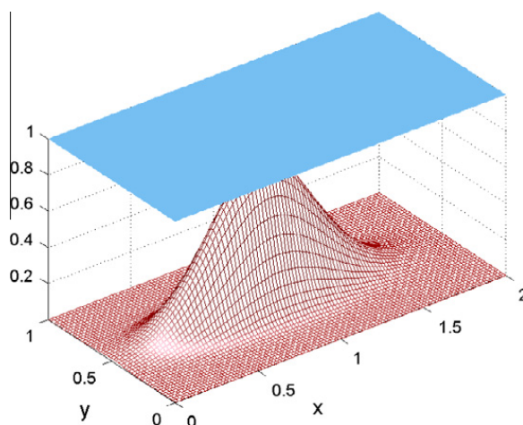
Fig. 11. Water level and bottom topography for the two-dimensional lake at rest.
