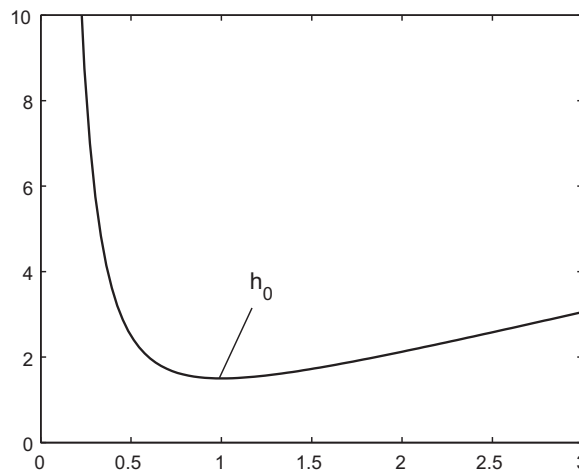
Fig. 6. The equilibrium variable p as a function of h for fixed values of b and m .
