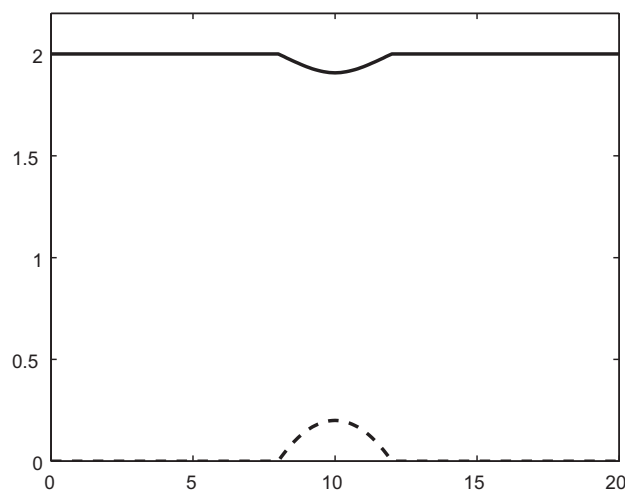
Fig. 7. Initial surface level for the subsonic steady state.
