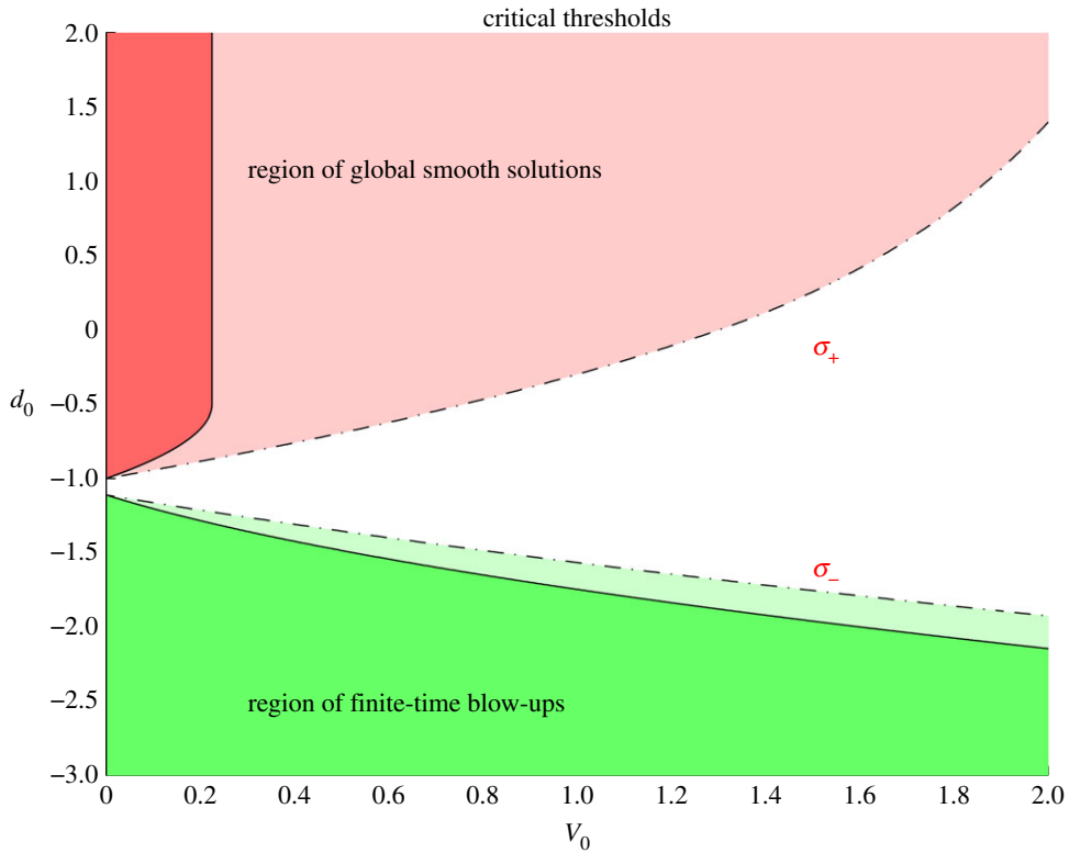
Figure 1. Illustration of the critical thresholds in one dimension. (Online version in colour.)
