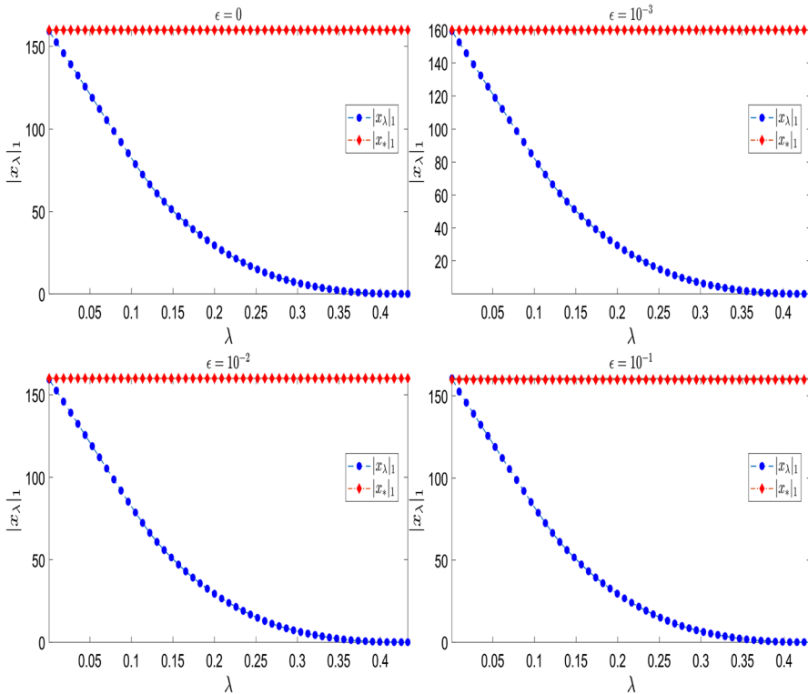
Fig. 2 \ell_1 norm of \mathbf{x}_\lambda approaches its upper bound |\mathbf{x}_*(k)|_1 as \lambda decreases
