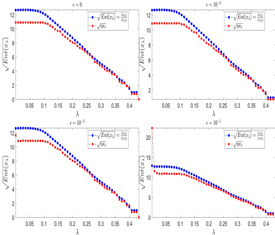
Fig. 4 Lower bounds of the re-scaled residual: (3.10) with \eta := \frac{1}{1+\delta} = 0.592 vs. the \ell_1 -entropy based (4.5)
