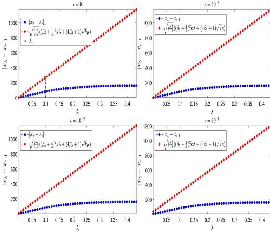
Fig. 5 \ell_1 -error for recovery of sparse data compared with the upper bound (4.12)
