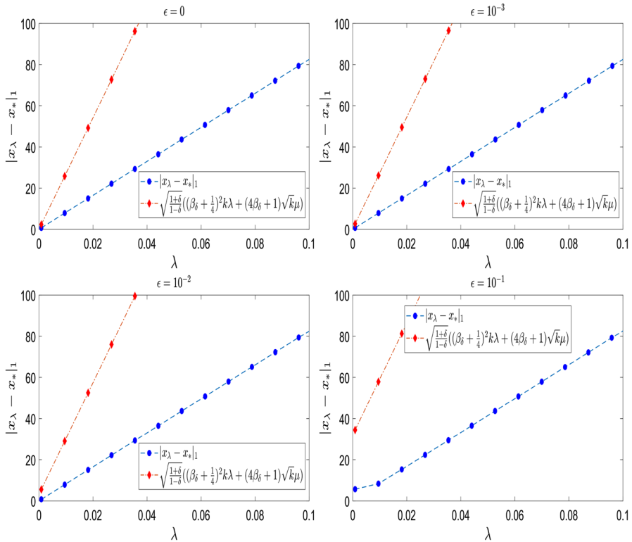
Fig. 6 The \ell_1 -error compared with the upper bound (4.12) zoomed near \lambda = 0
