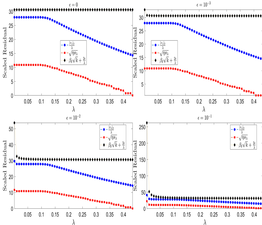
Fig. 3 Re-scaled residual \frac{|r_\lambda|_2}{\lambda} captured between its lower and upper bounds (3.10) and (3.2), \sqrt{\eta s_\lambda} \leq \frac{|r_\lambda|_2}{\lambda} \leq \beta_\delta \sqrt{k} + \frac{2\epsilon}{\lambda} \approx 30.61 with (\eta, \beta, \theta) = (0.59, 2.42, 0.1) corresponding to \delta = 0.7 . It peaks at a threshold value of 27, independent of the level of noise. When \lambda \ll \epsilon , there is an additional large term of order \frac{2\epsilon}{\lambda}
