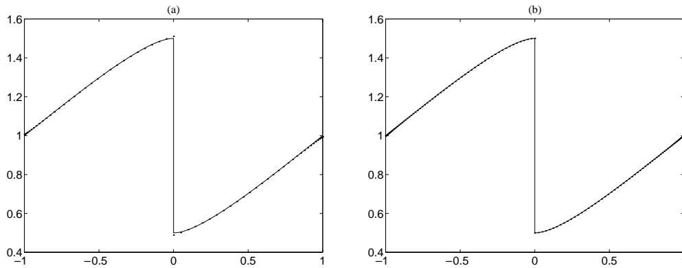
FIG. 4.3. The SV solution in Figure 4.1 after postprocessing.
