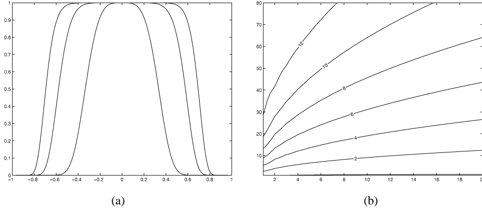
Fig. 2. (a) The Freud weight \exp(-c\xi^{2n}) with parameters (3.14) and \epsilon = 10^{-24} becomes increasingly wider for increasing n = 2, 4, and 6 . (b) Contour lines of \log_{10} \max |\Psi_l^n(\xi)| for \xi \in [-1, 1] with horizontal axis the weight order n and vertical axis the polynomial order l . Note that for l fixed, the maximum amplitude decreases as n increases.
