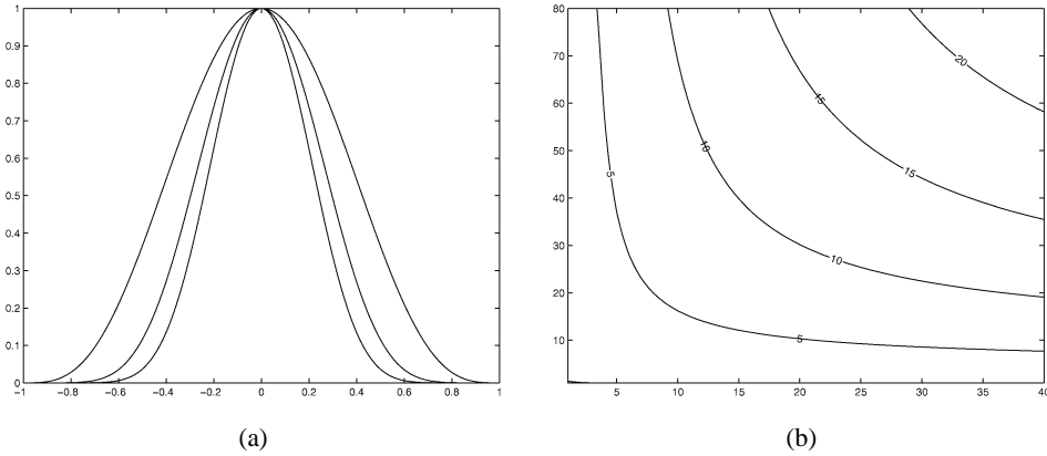
Fig. 1. (a) The Gegenbauer weight (1 - \xi^2)^{\lambda-1/2} becoming increasingly narrow for increasing \lambda = 4, 8, and 12 . (b) The amplitude of the Gegenbauer polynomials shown as contour lines of \log_{10} \max |\Phi_l^\lambda(\xi)| for \xi \in [-1, 1] . The horizontal axis represents the weight order \lambda , and the vertical axis represents the polynomial order l . Note the rapid increase in the polynomial amplitude for both parameters.
