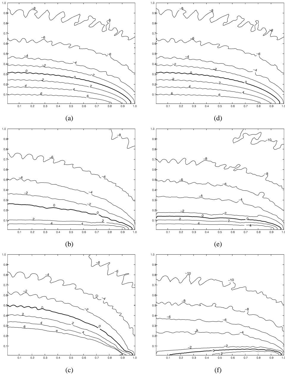
Fig. 4. The \log_{10} of the L^\infty[-1, 1] error in recovering f^{\text{symm,pole}} for z_s in the upper right quadrant of the complex plane, i.e., [\Re(z_s), \Im(z_s)] \in (0, 1] , from its truncated Fourier coefficients, with N = 64 (a, d), N = 128 (b, e), and N = 256 (c, f). \Re(z_s) and \Im(z_s) make up the respective horizontal and vertical axes. Results are from the Gegenbauer reprojection basis with \lambda = N/8 (left) and the Freud robust Gibbs complement (right) with parameters (3.14) where \epsilon = 10^{-24} . In each plot the thick contour line designating error of unit amplitude can be viewed as separating the region where an approximation is recovered from the region where the reconstruction fails. Note that the region for which the Gegenbauer reprojection fails to converge does not decrease with increasing N , whereas the Freud reprojection yields not only an increasingly accurate reconstruction, but also the region where the function is fully resolved from the given information is also increasing.
