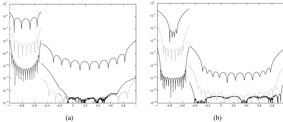
Fig. 5. The error in recovering f_2 using the (a) Gegenbauer and (b) Freud reprojection bases with the same parameters as in Fig. 4, except for the scaling by (b - a)/2 due to the length of the two intervals of smoothness, (-1, -1/2) and (-1/2, 1) . The given data were the global, taken over [-1, 1] , Fourier series, with N = 64 (upper solid), 128 (dotted), and 256 (lower solid).
