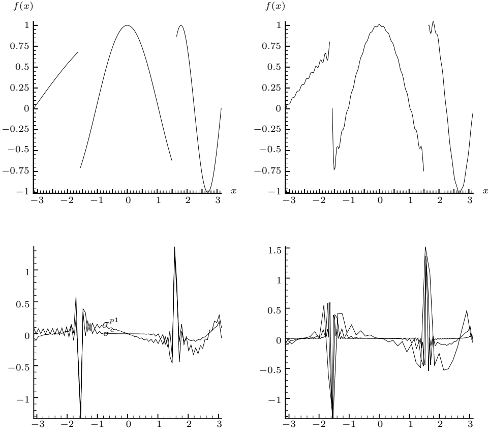
Figure 5.1. Top left: Piecewise smooth f(x) in (5.7). Top right: Gibbs phenomenon for S_{40}f(x) . Bottom left: Edge detection in S_{40}f using K_{40}^{\sigma}f , comparing the exponential concentration factors \sigma_{\text{exp}}(\xi) = \exp(\frac{1}{6\xi(\xi-1)}) vs Fejér factors \sigma(\xi) = \xi . Bottom right: Exponential concentration K_N^{\sigma_{\text{exp}}} f(x) with N = 20, 40, 80 modes. Observe that the root-exponential decay of K_{80}^{\sigma_{\text{exp}}} f(x) becomes almost flat when x is well inside the intervals of smoothness of f , which are well separated from the neighbourhoods of the edges.
