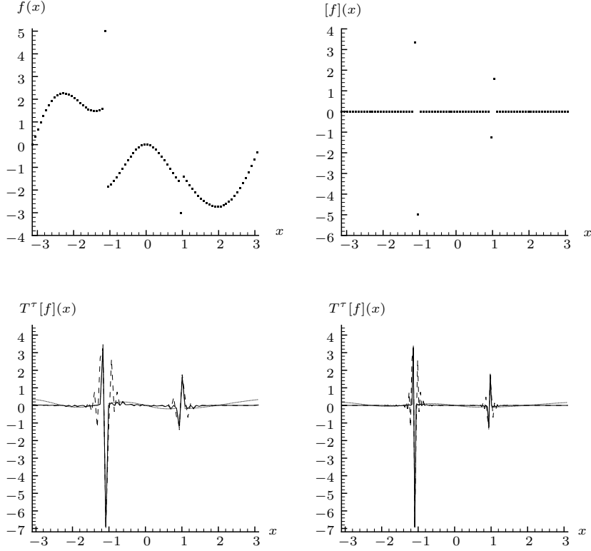
Figure 7.2. Top left: Piecewise f with adjacent edge. Top right: K_{80}^{\sigma_{\text{mm}}} f(x) . Bottom left: Edge detection using first-order I_N^{\tau_{\text{pol}}} f(x) (dotted), I_N^{\tau_{\text{exp}}} f(x) (dashed) and the I_N^{\tau_{\text{mm}}} f(x) algorithm (solid) with N = 80 grid-points. Bottom right: The same with N = 160 points.
