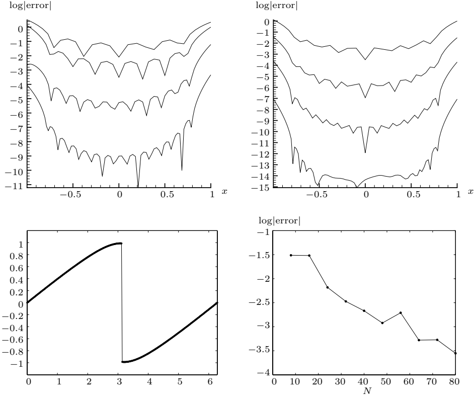
Figure 10.4. Top : Error in log-log scale of the Gegenbauer reconstruction G_p^{(\alpha)}(S_N f)_\pi(x) with N = 16, 24, 36 and 52 modes for f(x) = \cos(1.4\pi(x-1)) , x \in (-1, 1) . Top left : \alpha_N = p_N = N/4 . Top right : \alpha_N = p_N = N/5 . Bottom left : Gegenbauer reconstruction of I_{40}f(x) , where I_N f = u_N(x, t = 1.5) is a steady discontinuous solution of the inviscid Burgers equation, computed using a smoothed pseudo-spectral Fourier projection, \partial_t u_N(x_\nu, t) + \partial_x \left( \frac{I_N(u_N)^2}{2} \right)(x_\nu, t) = 0 and subject to u_N(x_\nu, t = 0) = \sin(x_\nu) . Bottom right : Log-log plot of the error.
