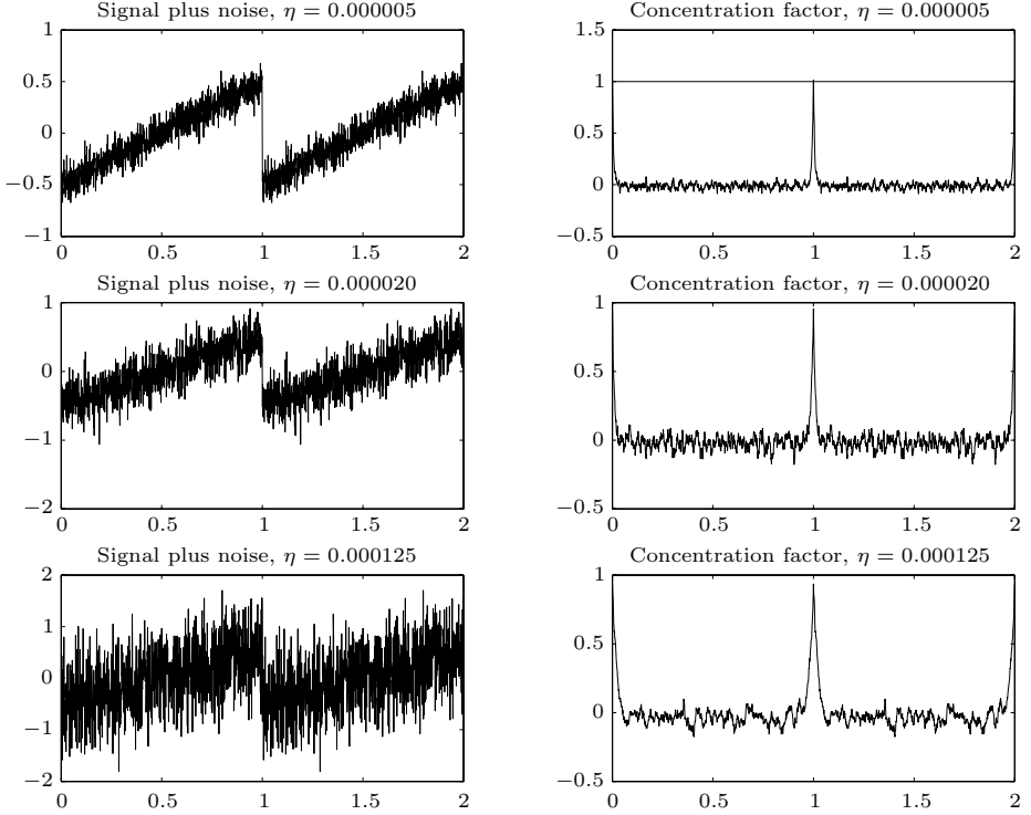
Figure 6.2. Detection of edges in noisy sawtooth function corrupted with various values of \eta , using the concentration kernel (6.21a) with \beta = 1/8\sqrt[3]{\eta} .
