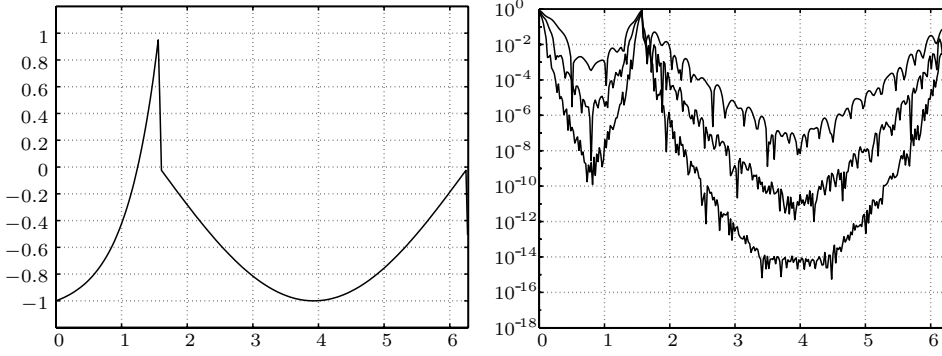
Figure 10.1. Left: Function f(x) in (10.12). Right: Log-error of its reconstruction from S_N f , N = 32, 64, 128 using the adaptive mollifier \Phi_{p_N, \delta} in (10.10a) with p_N = d_x N / \sqrt{e} .
