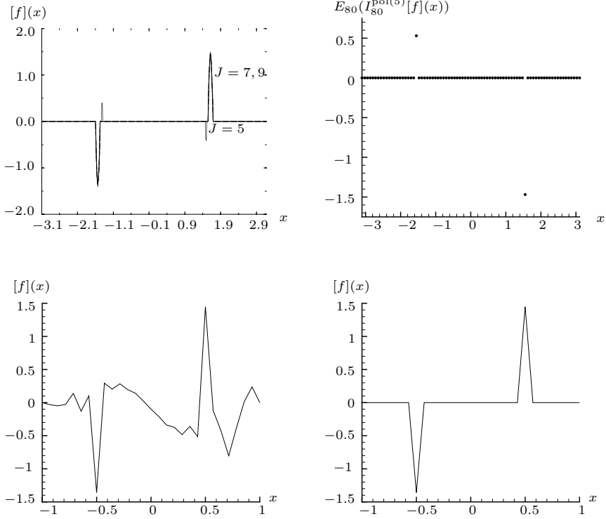
Figure 7.1. Top left : Jump value obtained by K_{40,J_c}^\sigma f for f(x) in (7.1) with q = 1 and \sigma(\xi) = \sin(\xi) . Top right : I_{80,J_c}^\tau f with \tau(\xi) = \xi^5 in (7.2). Bottom : Detection of edges in Chebyshev expansion of f(x/\pi) before and after enhancement with q = 1 and J_c = 5 .
