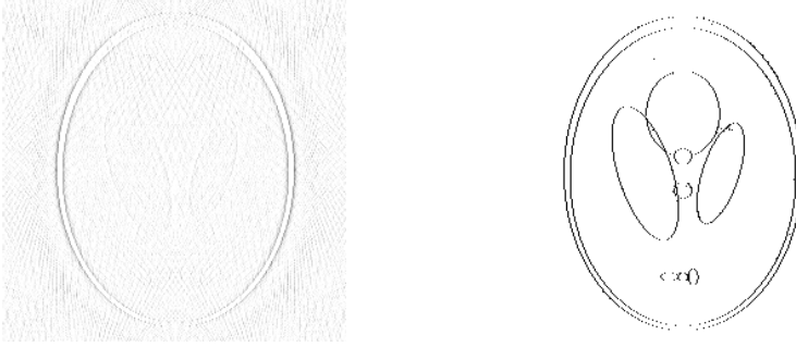
Figure 8.3. Recovered phantom image from incomplete spectral data. Left : Result by the back projection. Right : Recovered edges of Shepp phantom graph by compressive sensing edge detection.
