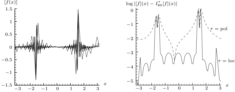
Figure 6.1. Left : Detection of edges in the interpolant of f in (5.7) using polynomial concentration factors, I_N^{\tau_2} f , with N = 20, 40 and 80 modes. Right : Logarithmic error of the fifth-order local trigonometric vs the global polynomial concentration factors I_{80}^{\tau_5} f(x_\nu) .
