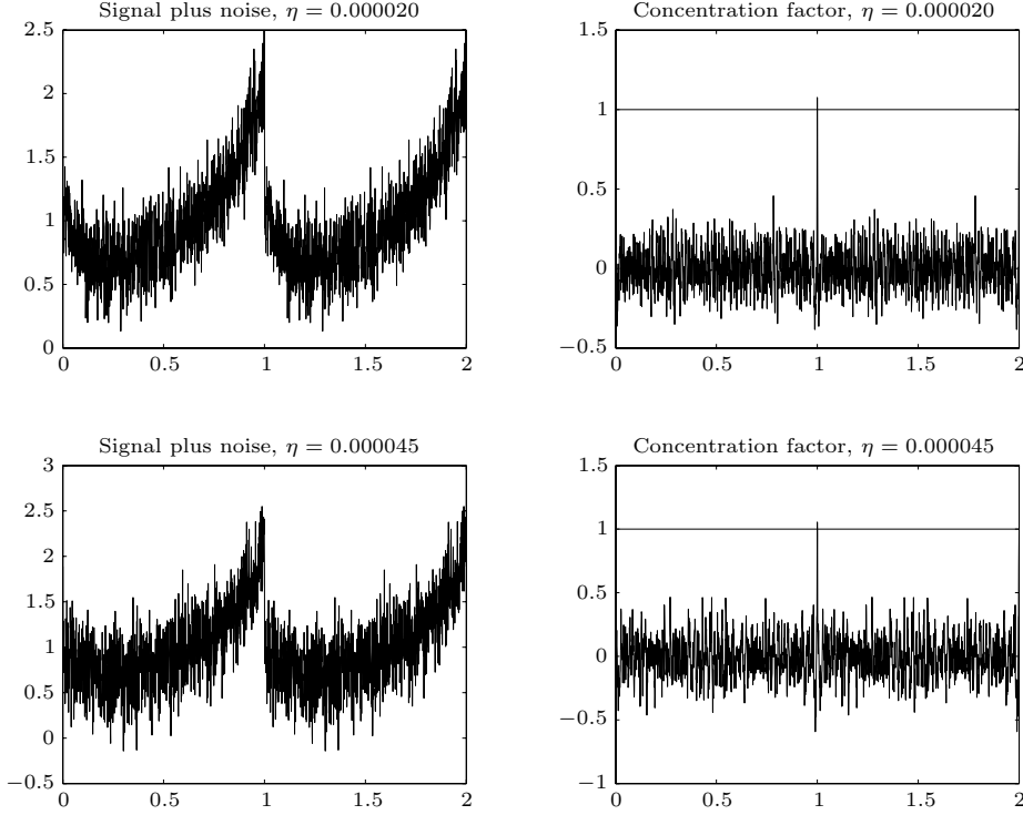
Figure 6.3. Detection of edges in noisy sawtooth function corrupted with various values of \eta , using the concentration factors (6.22) with \beta = 1/8\sqrt[3]{\eta} .
