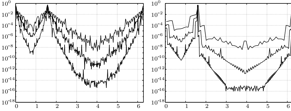
Figure 10.3. Left : Log-error of reconstructing f from S_N f , N = 32, 64, 128 using the 4th-order normalized adaptive mollifier (10.21c) with p_N = d_x N / \sqrt{e} . Right : Reconstruction of f from its discrete data, I_N f , N = 32, 64, 128 , using the 4th-order normalized mollifier (10.23).
