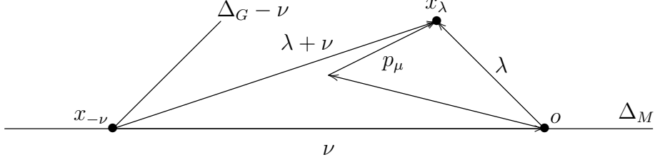
FIGURE 1. The broken path p_\mu from o to x_\lambda is an LS path of type \mu . Then the Littelmann bigon with the sides p_\mu and \overline{ox_\lambda} yields a Littelmann triangle with the geodesic sides \overline{x_{-\nu}o} , \overline{x_{-\nu}x_\lambda} and the broken side p_\mu .
